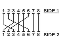
Figure A-1: Straight-through and Crossover Cables
