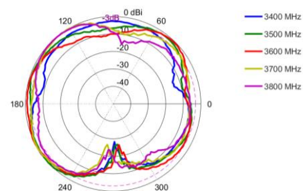
Azimuth: 3400 – 3800 MHz
